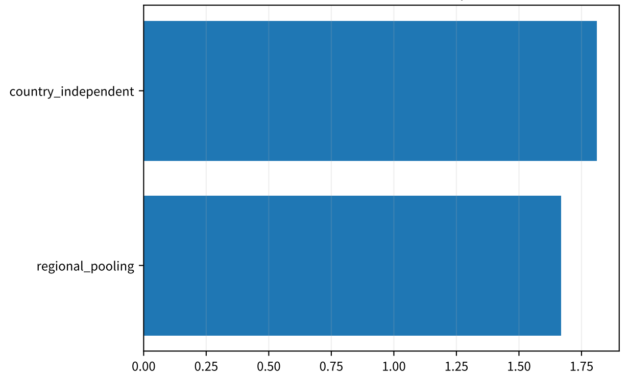
CommonQ5MinusQ1MaxDrawdown
