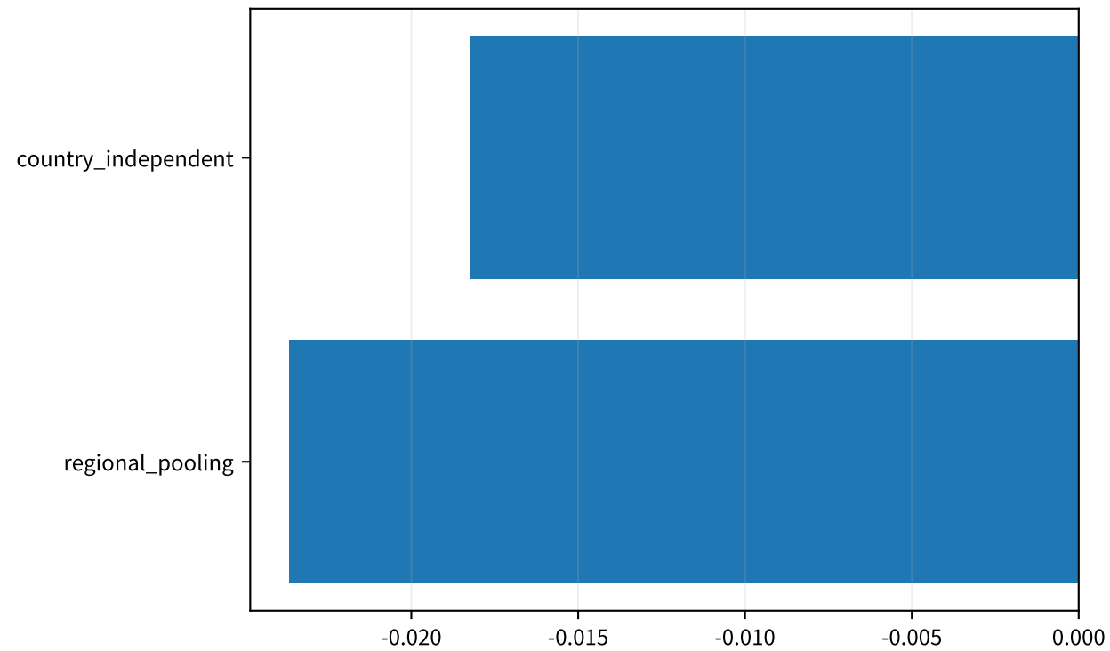
CommonQ5MinusQ1MaxDrawdown
