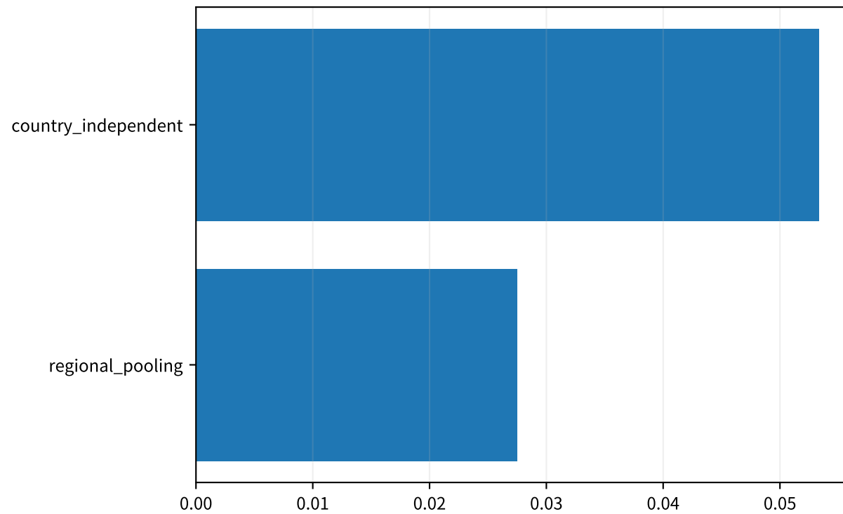
CommonQuintileMonotonicity
